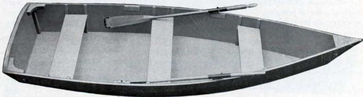
KENNEBEC FISHERMAN, 12 feet, Interior
